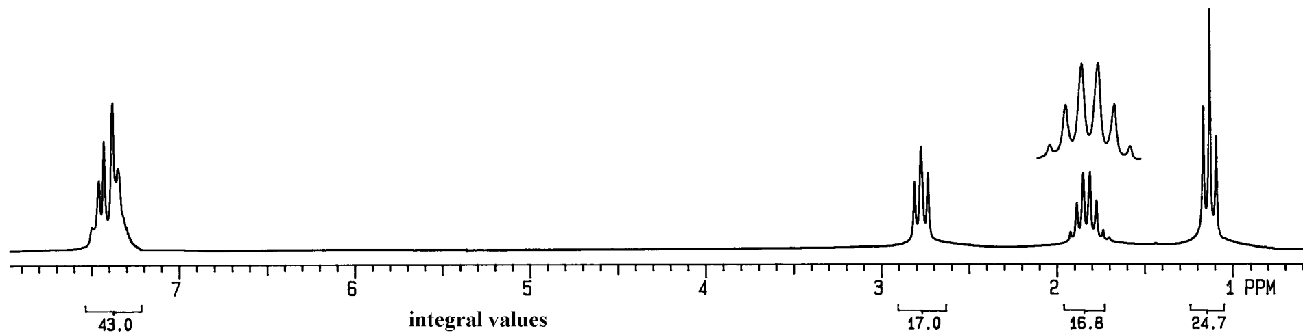
Proton NMR
