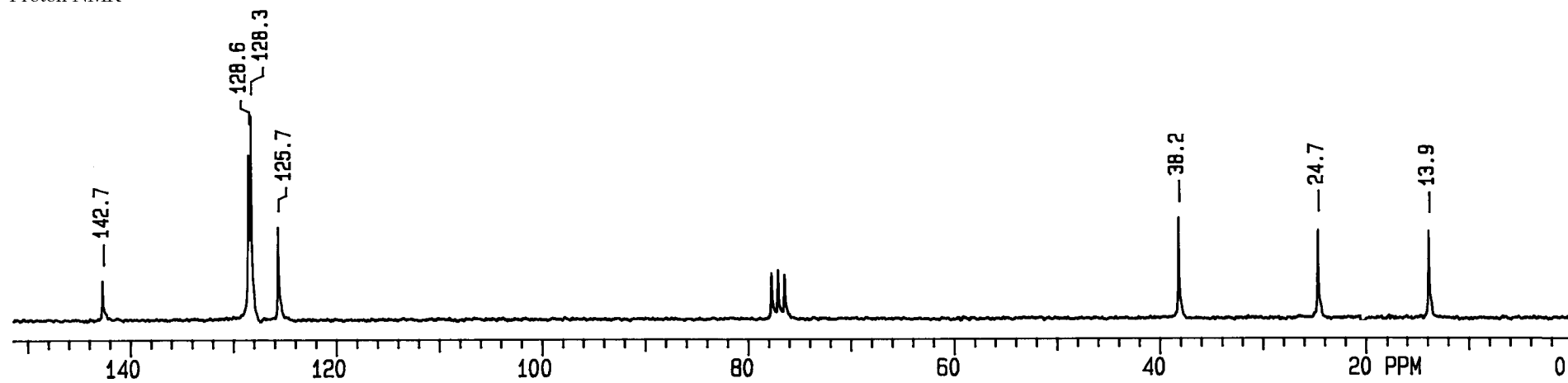
Carbon 13 NMR
