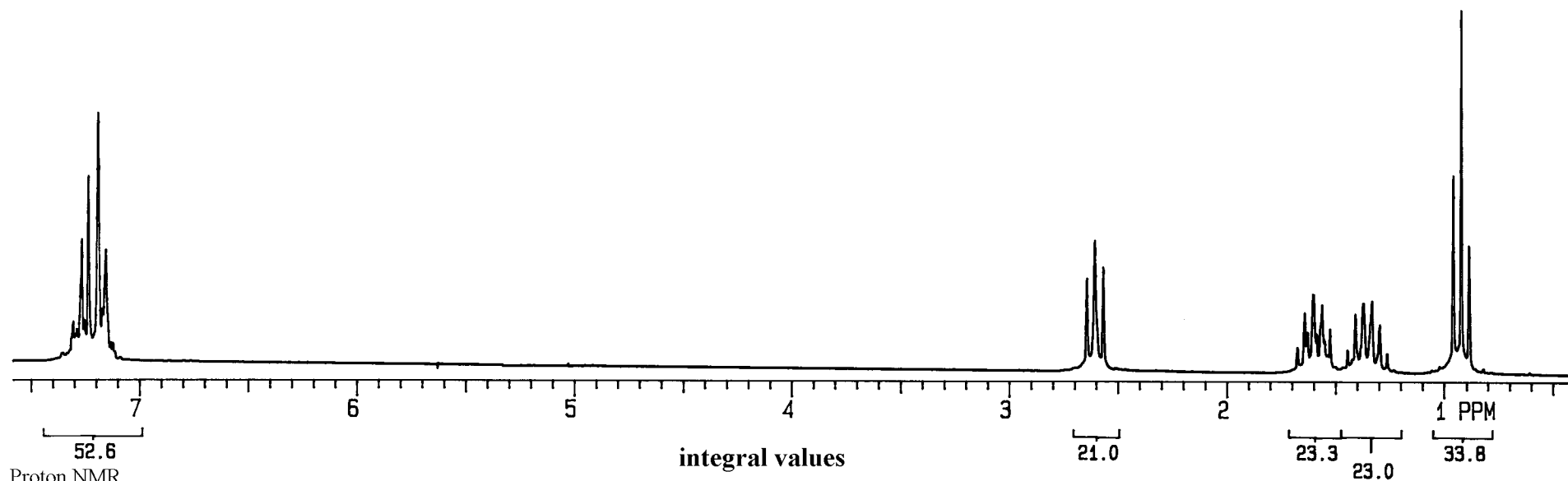
Proton NMR
