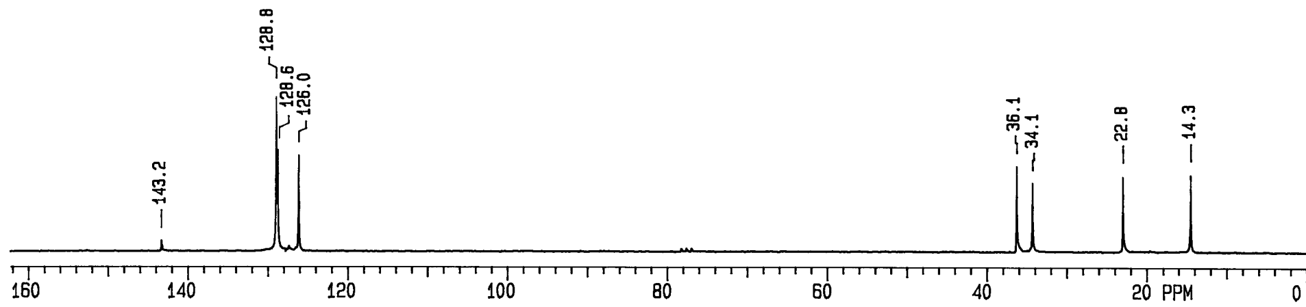
Carbon 13 NMR
