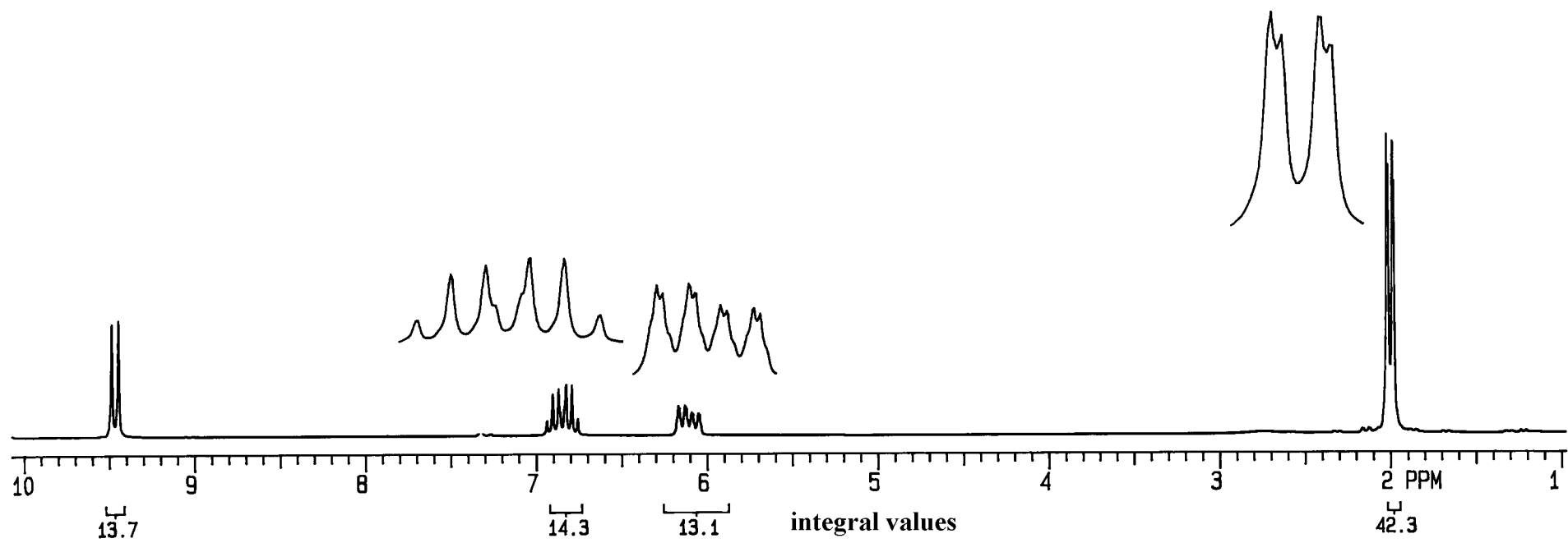
Proton NMR
