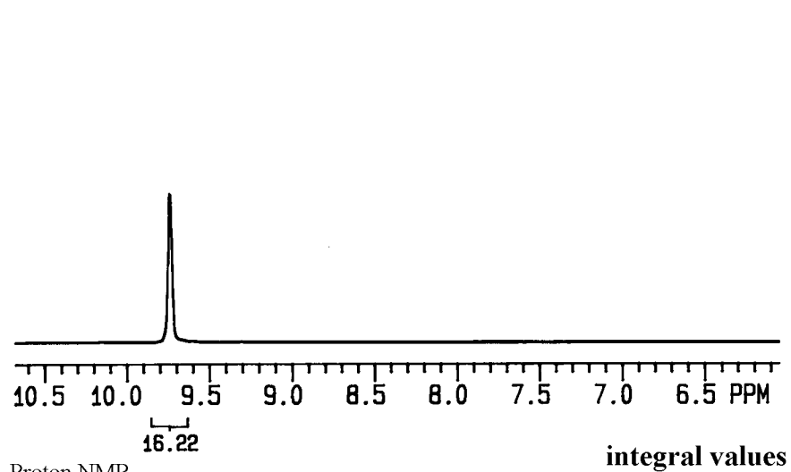
Proton NMR
