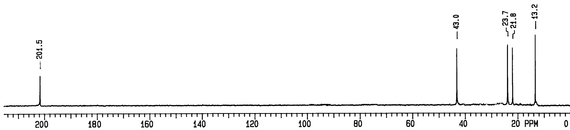
Carbon 13 NMR
