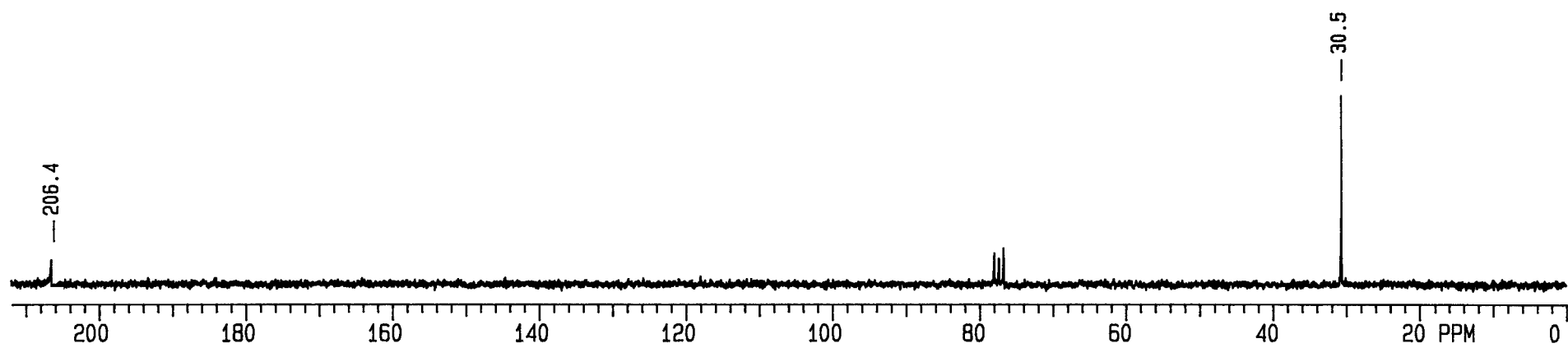
Carbon 13 NMR
