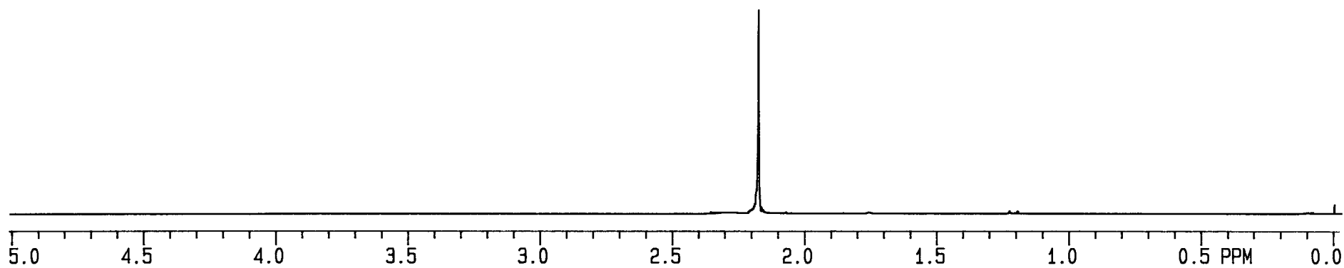
Proton NMR
