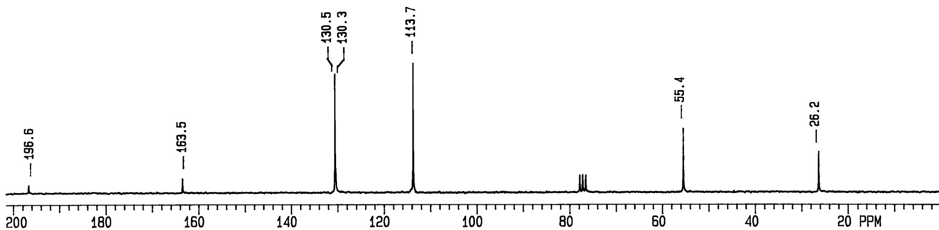
Carbon 13 NMR
