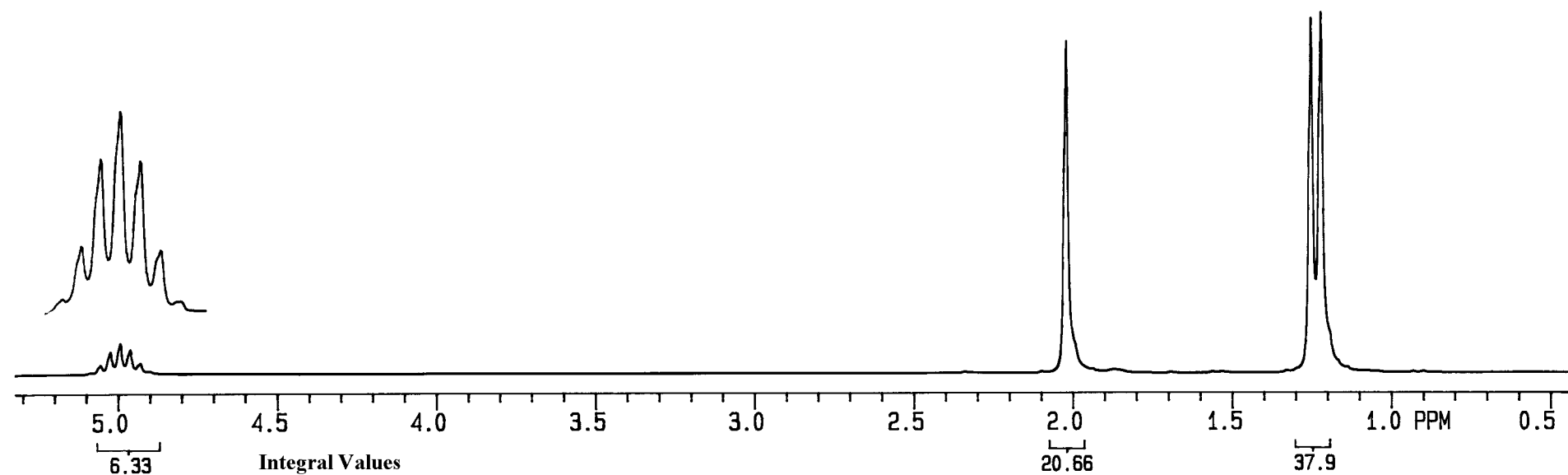
Proton NMR
