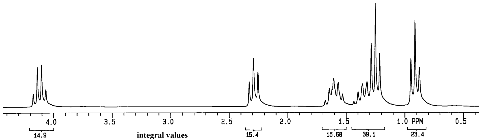
Proton NMR
