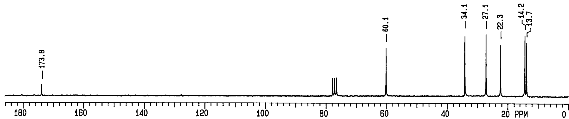
Carbon 13 NMR
