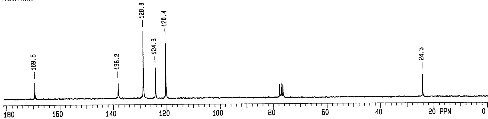
Carbon 13 NMR
