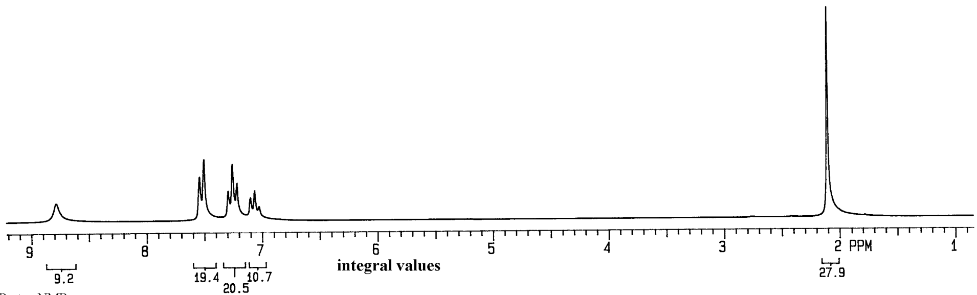
Proton NMR
